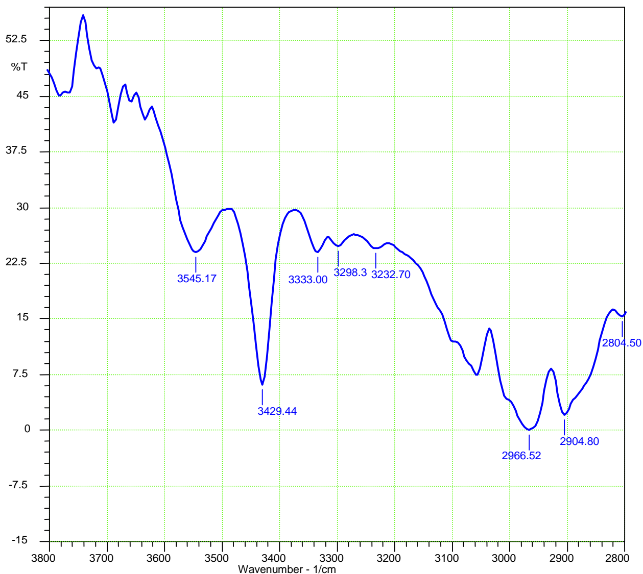
Figure 12. ATR FT-IR spectrum of APTES on ITO in the range of 3800\text{-}2800\text{ cm}^{-1} .
