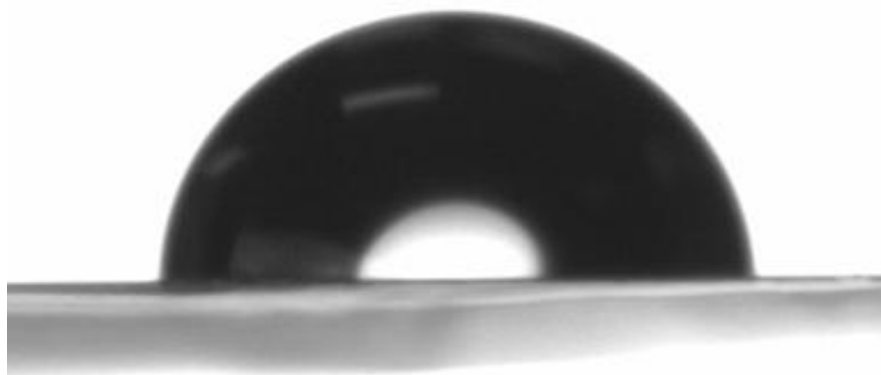
Figure 9. Micrograph of water contact angle on SAM surface (experimental data).
