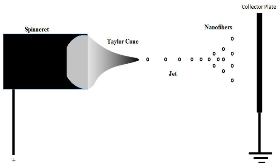
Figure 2.3. Taylor Cone
